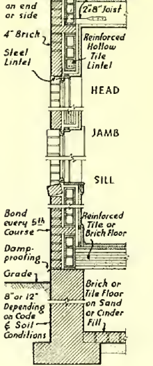
Wall Section
